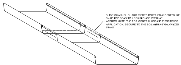
CG-2 CONNECTION NOT TO SCALE
