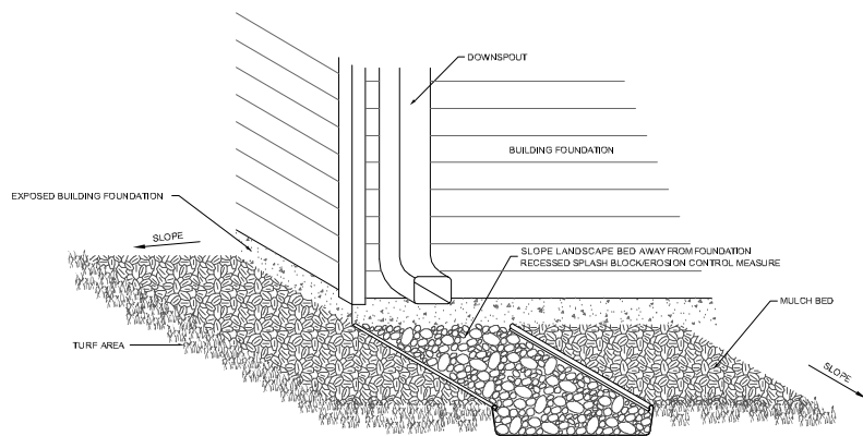
CG-4 DOWNSPOUT APPLICATION NOT TO SCALE
