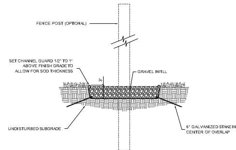
CG-3 FENCE APPLICATION NOT TO SCALE
