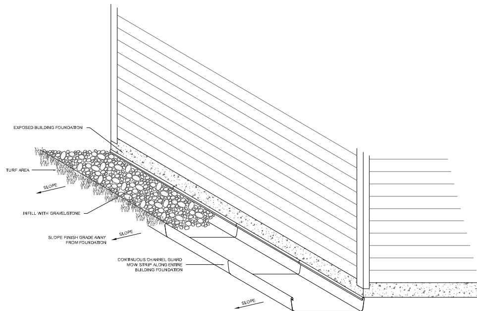
CG-5 MOW STRIP APPLICATION NOT TO SCALE
